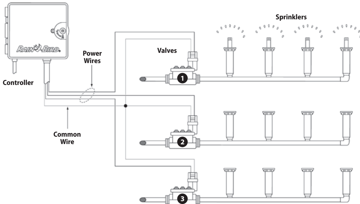
Figure A.2 - LXME System Wiring Diagram
