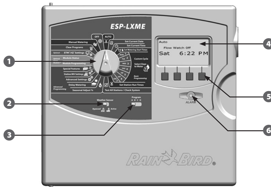
Figure A.1 - ESP-LXME Controller Front Panel Features
