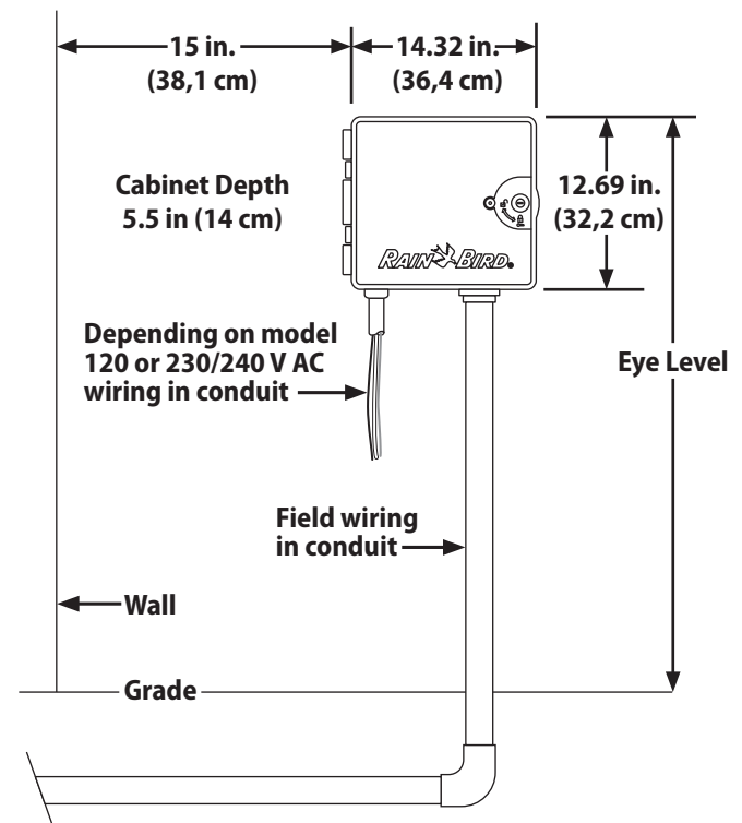
Figure H.2 - Select Controller Location
